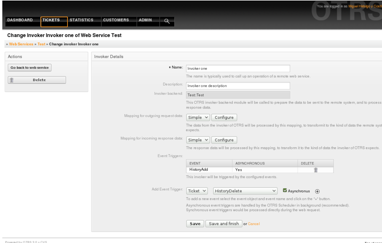
Figure: Web service invoker.
